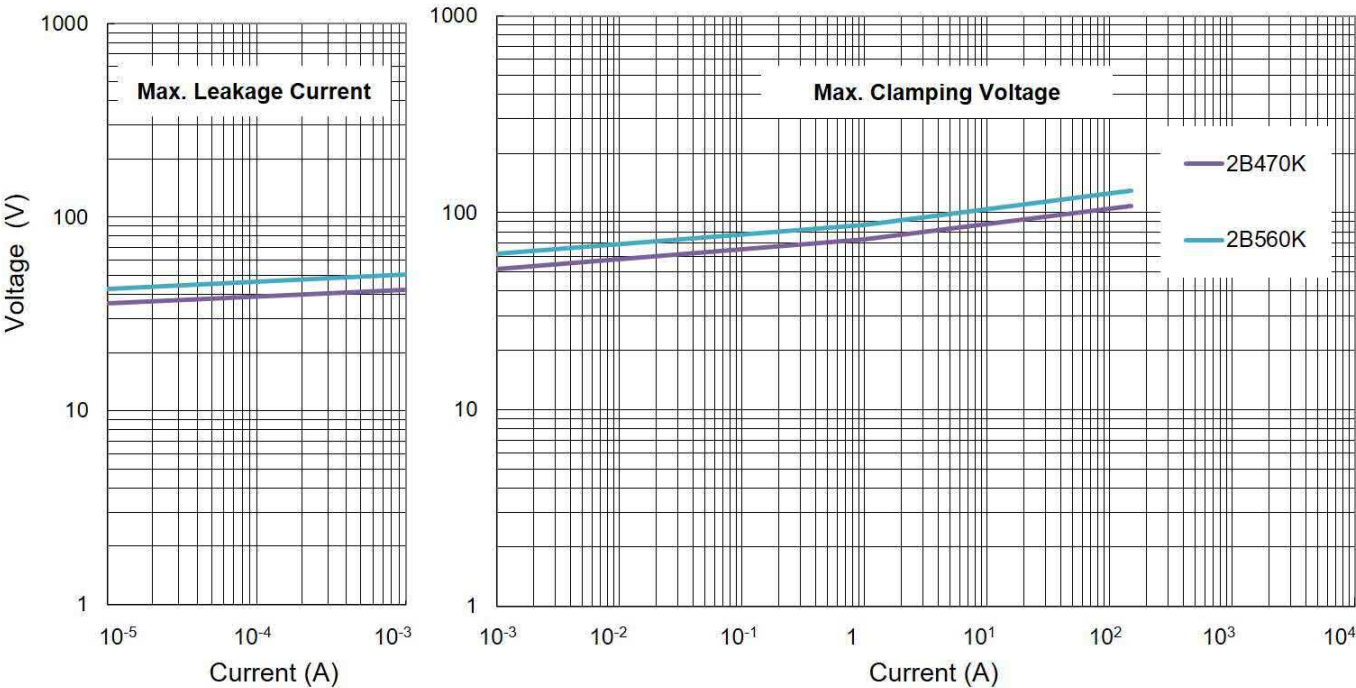
Max. Leakage Current and Max. Clamping Voltage Curves (TVM3B270K~TVM3B680K)
